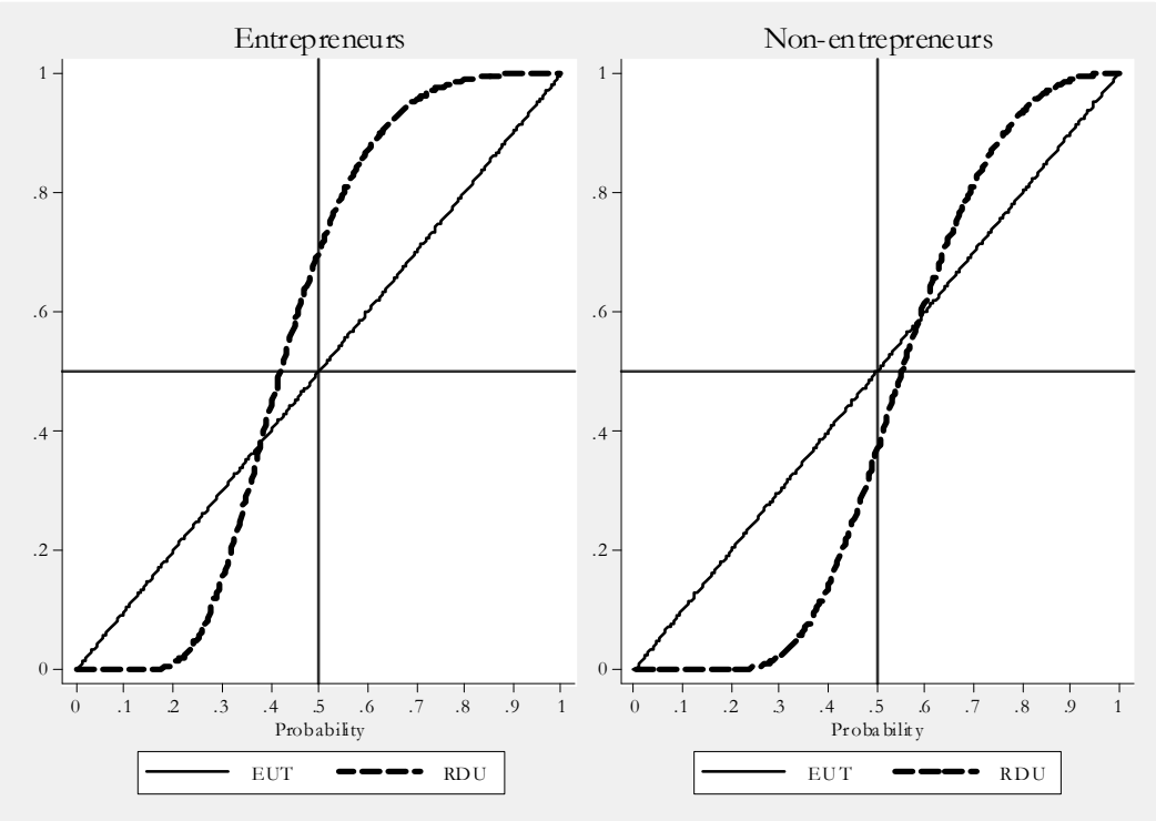
Figure 1. Prelec Probability Weighting Function
